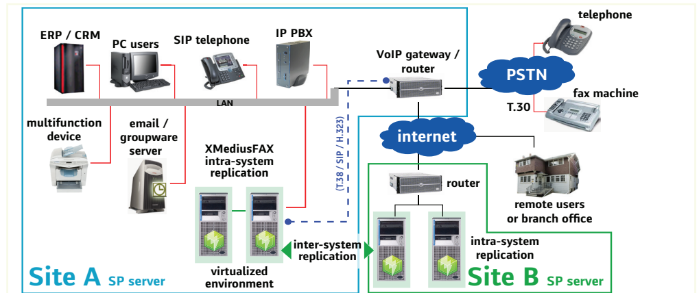
XMediusFAX SP Edition Typical Implementation
